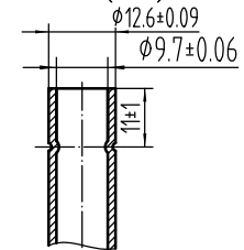
吸气管放大图 Suction Tube(Scaled)
