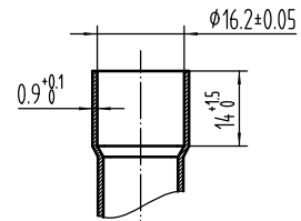
吸气管放大图 Suction Tube(Scaled)
