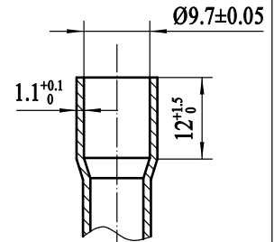
吸气管放大图 Suction Tube (Scaled)
